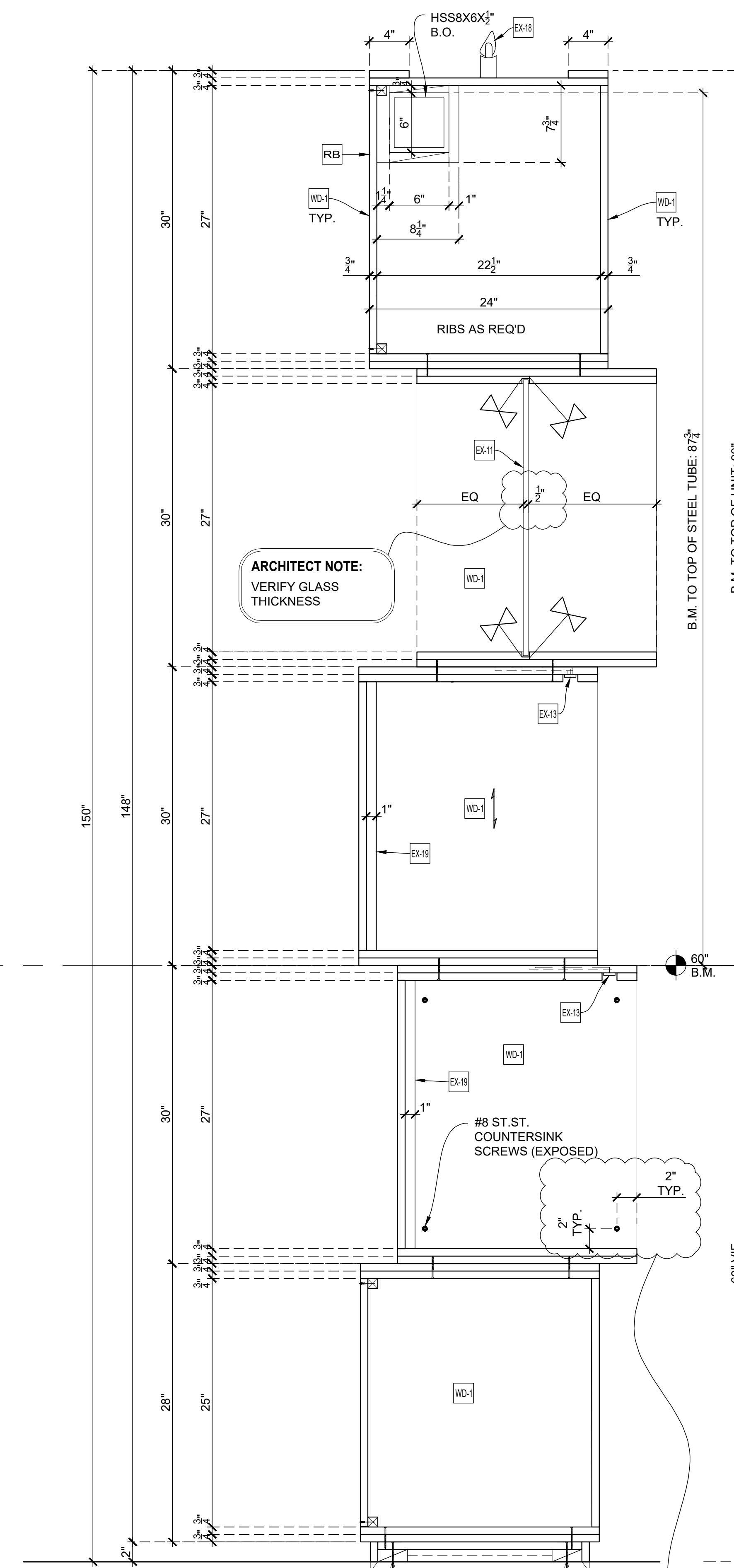
VERTICAL SECTION SCALE: 1-1/2" = 1'-0" Arch't Ref.: 1C/A-845.00
